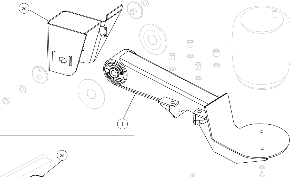
Winged, Weld-on Frame Bracket with QUIK-ALIGN
